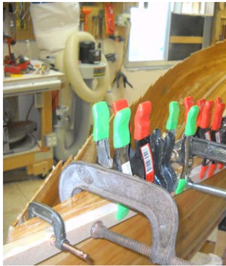
May 30 Week 6 installing the gunwale hardwood framing ( 68 clamps )
